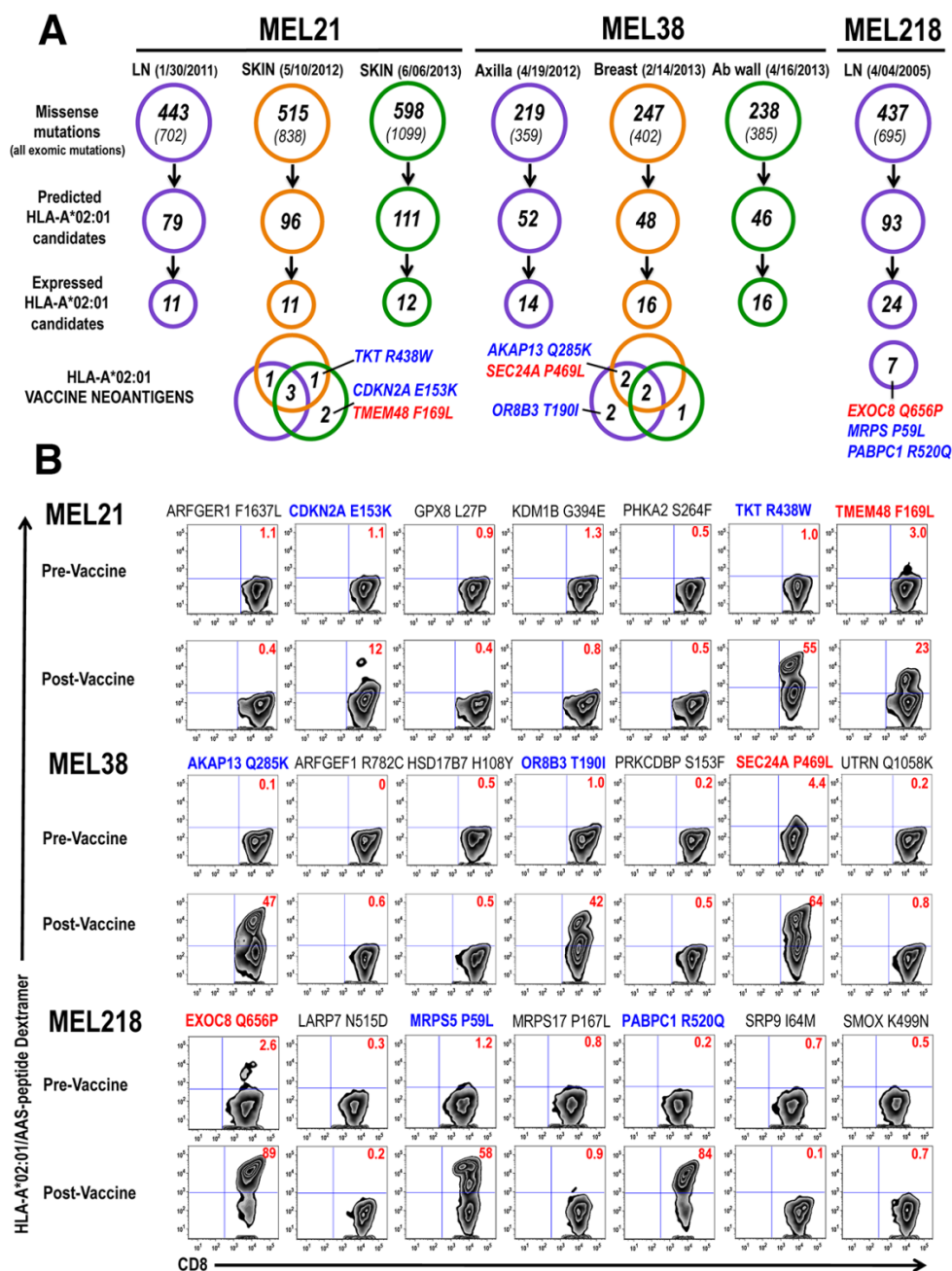
Fig. 1. Vaccine candidate identification and immune monitoring. (A) Distribution of somatic (exomic and missense) mutations identified in patients MEL21 and MEL38 metachronous tumors (anatomical location and date of collection indicated) and patient MEL218 tumor are shown. HLA-A*02:01-binding candidate peptides were in silico identified among AAS and expression of gene encoding mutated protein determined from cDNA capture data (tables S1 to S3). Venn diagrams show expression, among metachronous tumors, of mutated genes encoding vaccine neoantigens. The identities of the 3 immunogenic neoantigens identified in each patient are depicted in diagrams; color coding identifies naturally occurring (red) and vaccine-induced (blue) neoantigens. (B) Immune-monitoring of neoantigen-specific CD8 + T cell responses. Results are derived from PBMC isolated before DC vaccination (Pre-vaccine) and at peak (Post-Vaccine). PBMCs were cultured in vitro in the presence of peptide and IL-2 for 10 days followed by HLA-A*02:01/AAS-peptide dextramer assay. This immune monitoring strategy allows the reliable detection, as well as, the assessment of replicative potential of vaccine-induced T cell responses (fig. S4A). Color coding according to (A), numbers within dot plots represent percent neoantigen-specific T cells in lymph + /CD8 + gated cells.
